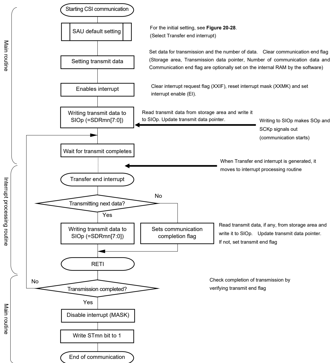
Figure 20-32. Flowchart of Master Transmission (in Single-Transmission Mode)
