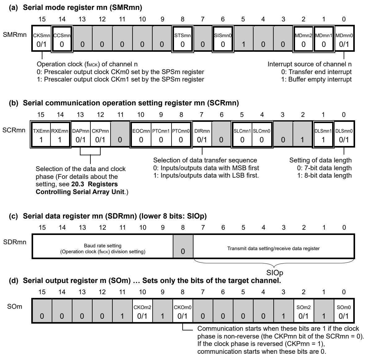
Figure 20-43. Example of Contents of Registers for Master Transmission/Reception of 3-Wire Serial I/O (CSI00, CSI10, CSI30) (1/2)
