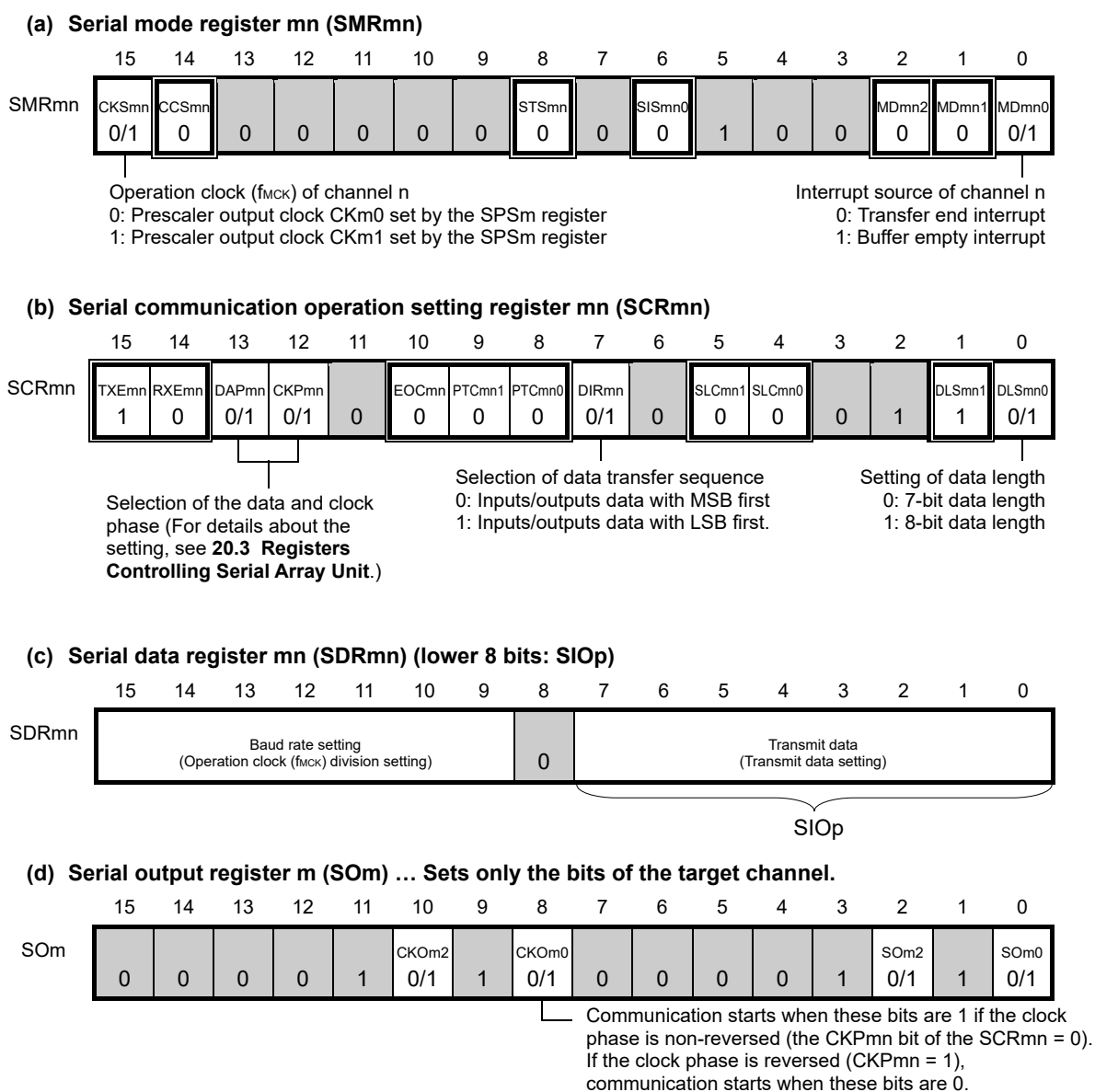
Figure 20-27. Example of Contents of Registers for Master Transmission of 3-Wire Serial I/O (CSI00, CSI10, CSI30) (1/2)
