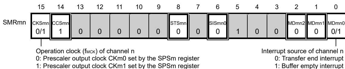
Figure 20-51. Example of Contents of Registers for Slave Transmission of 3-Wire Serial I/O (CSI00, CSI10, CSI30) (1/2)
