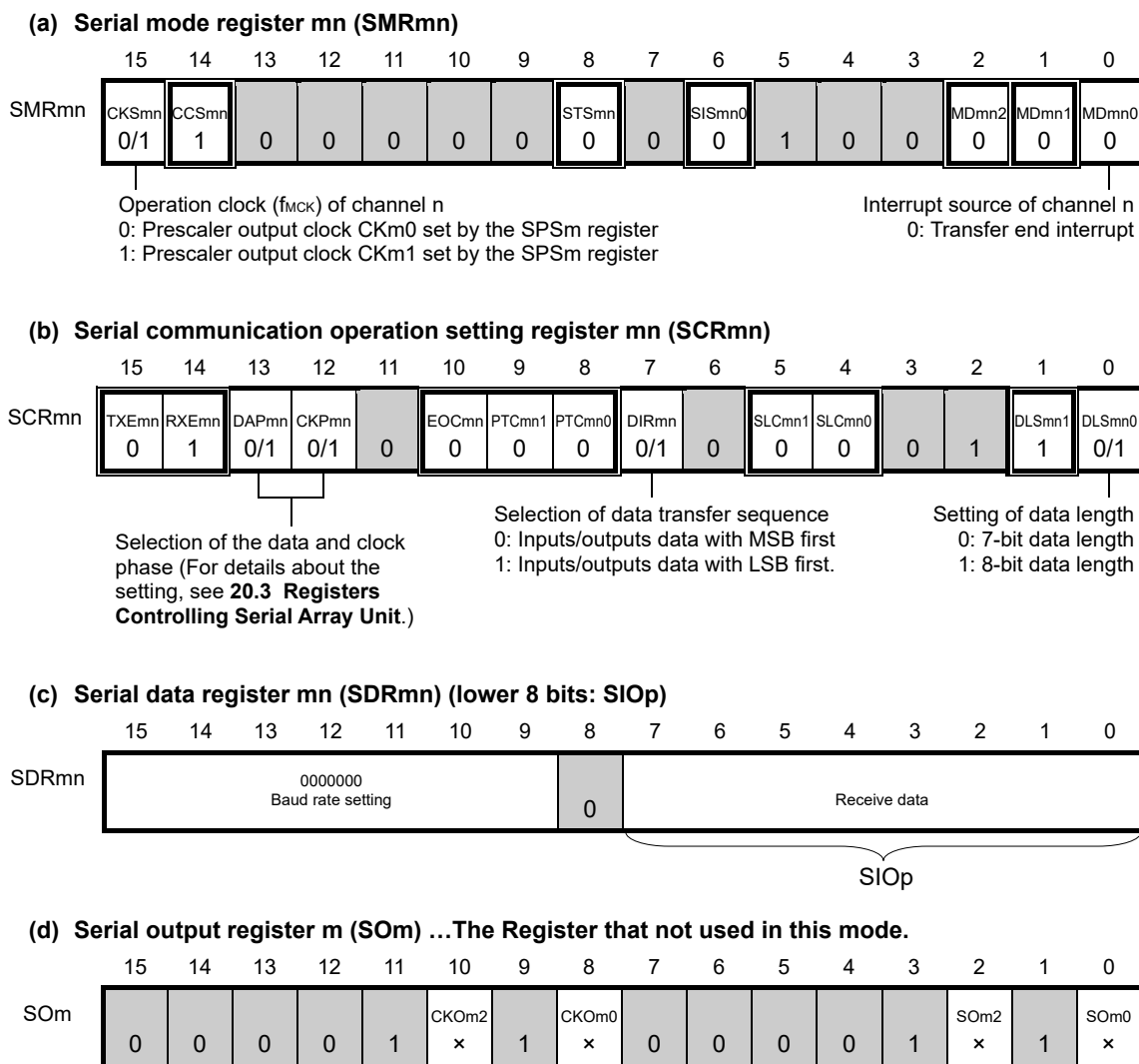
Figure 20-59. Example of Contents of Registers for Slave Reception of 3-Wire Serial I/O (CSI00, CSI10, CSI30) (1/2)
