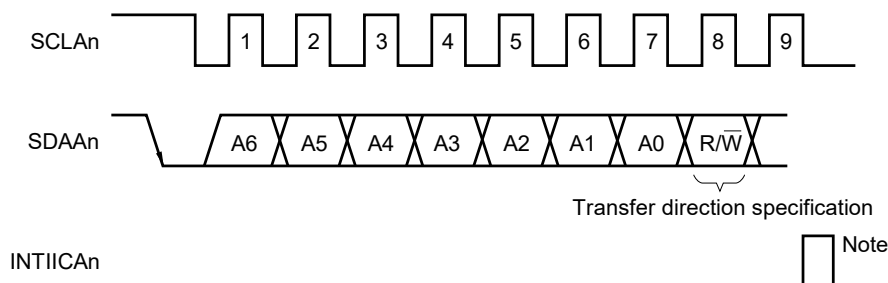
Figure 21-18. Transfer Direction Specification
