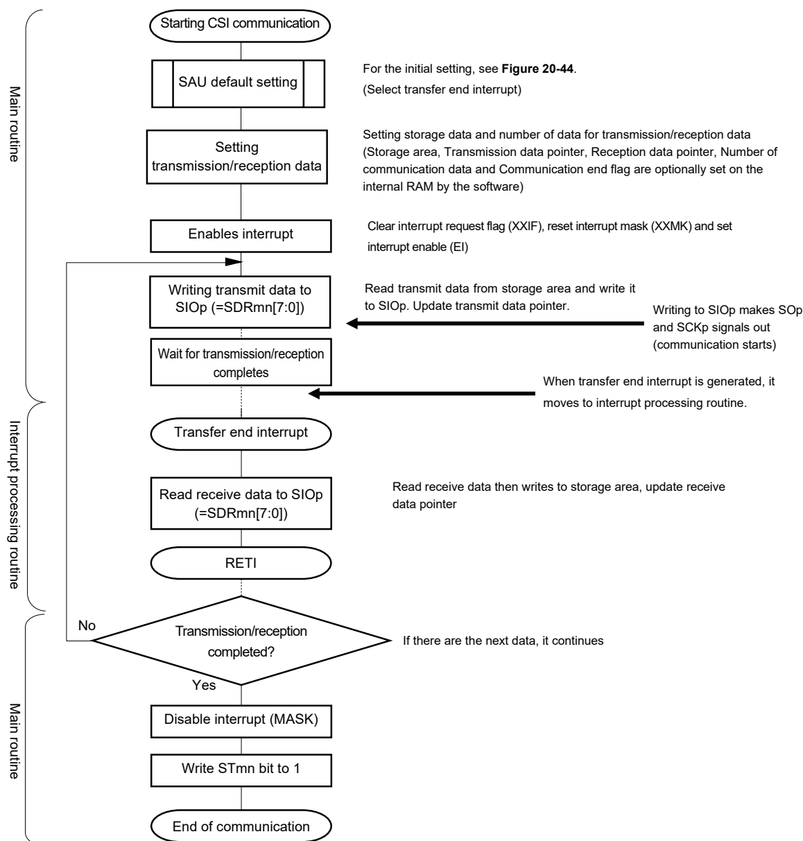
Figure 20-48. Flowchart of Master Transmission/Reception (in Single-Transmission/reception Mode)
