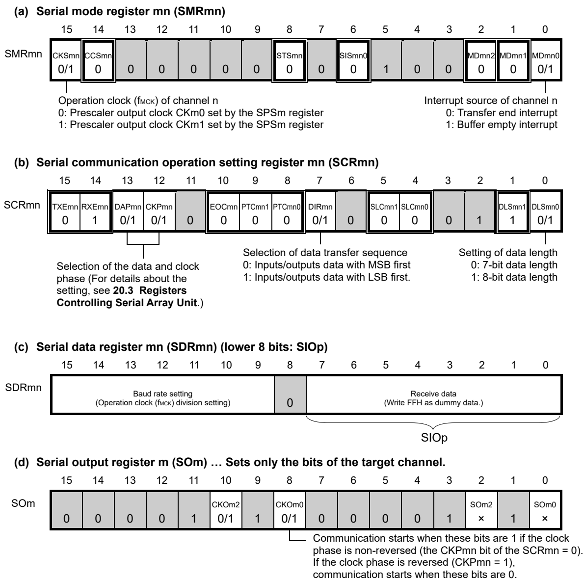
Figure 20-35. Example of Contents of Registers for Master Reception of 3-Wire Serial I/O (CSI00, CSI10, CSI30) (1/2)
