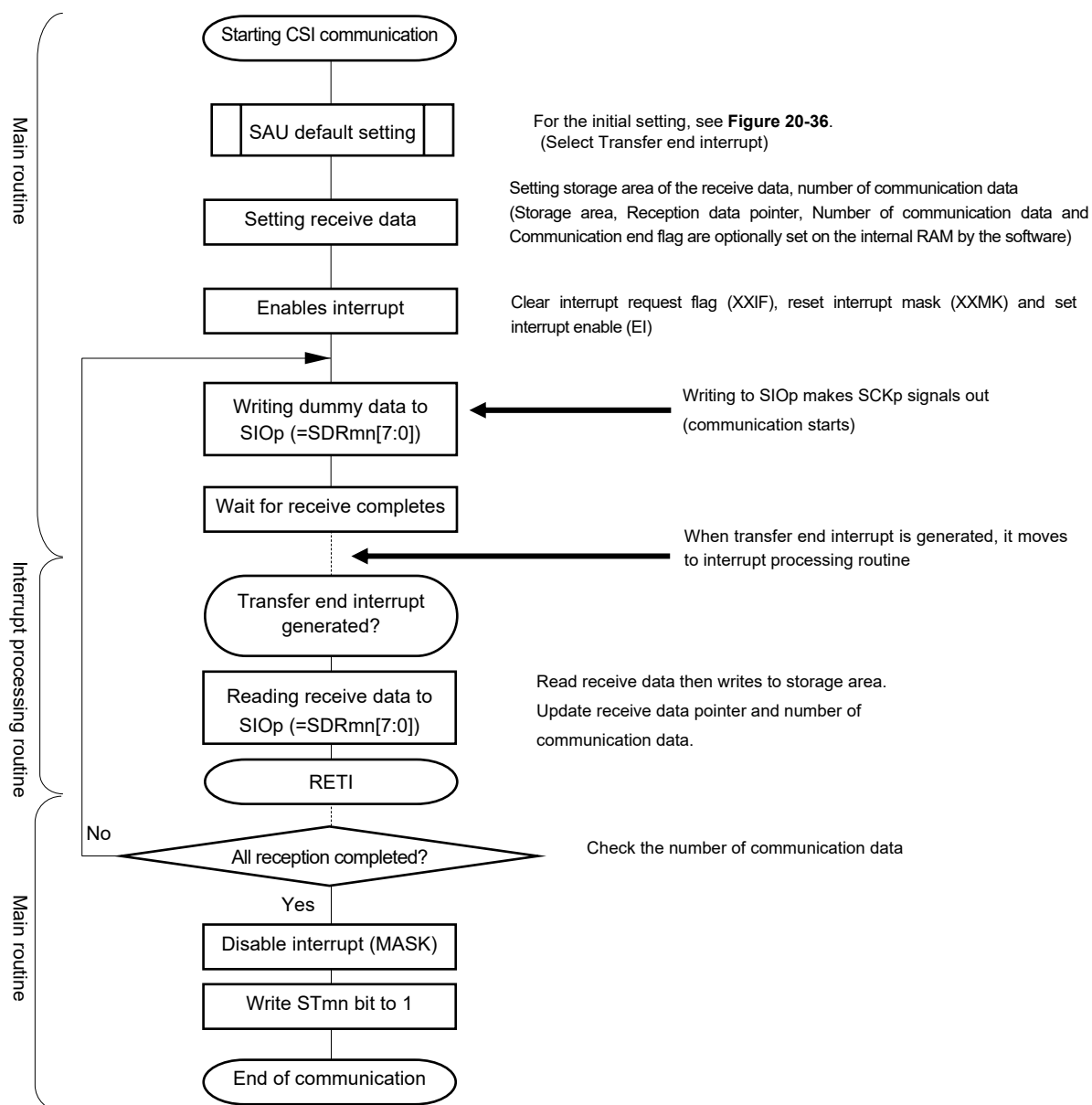
Figure 20-40. Flowchart of Master Reception (in Single-reception Mode)
