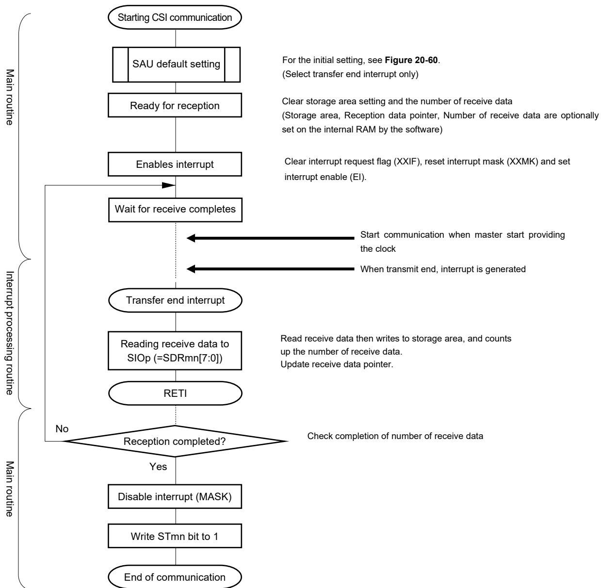
Figure 20-64. Flowchart of Slave Reception (in Single-reception Mode)
