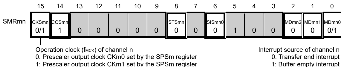
Figure 20-65. Example of Contents of Registers for Slave Transmission/Reception of 3-Wire Serial I/O (CSI00, CSI10, CSI30) (1/2)
