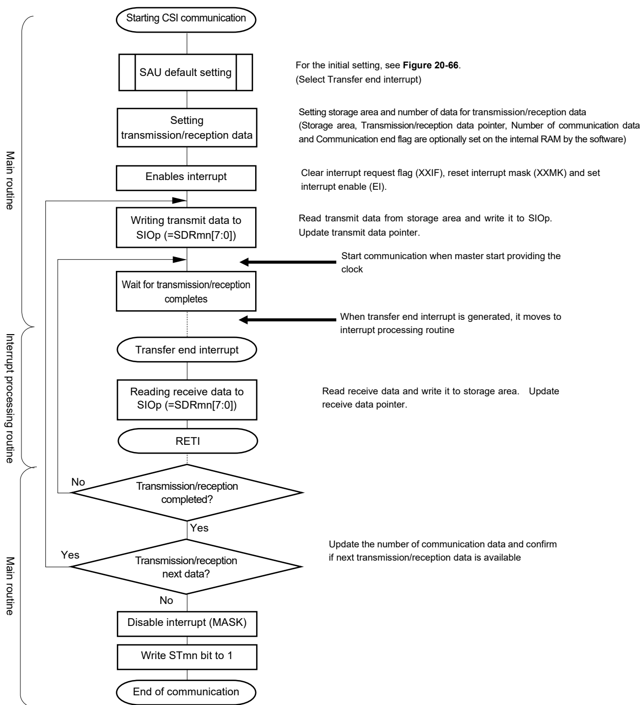
Figure 20-70. Flowchart of Slave Transmission/Reception (in Single-Transmission/Reception Mode)
